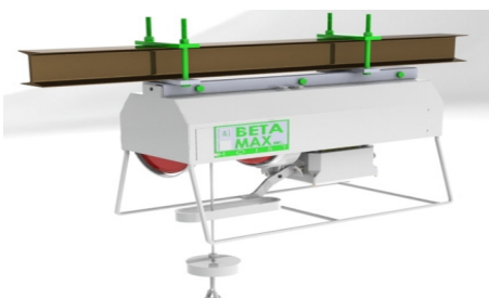
Fixed I-Beam
