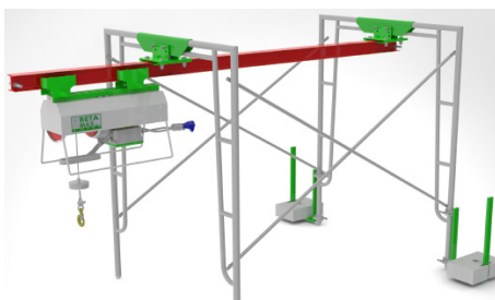
I-Beam Trolley
