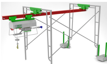
I-Beam Trolley
