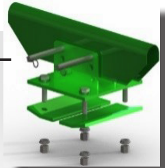
Suspension Bracket
